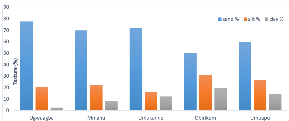
Fig. 1. Bar chart showing the texture classification of the different soil samples.
