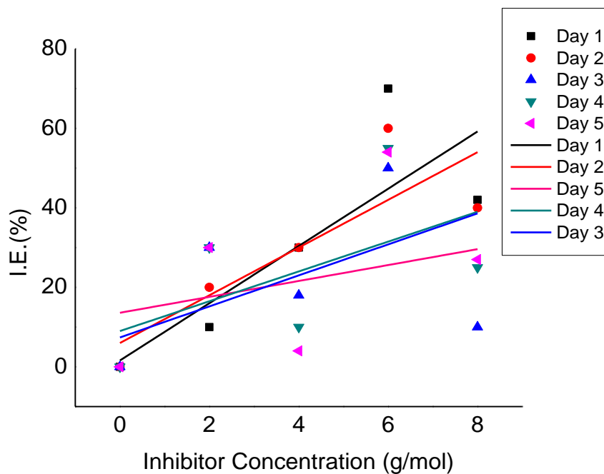
Figure 1. Effect of the amount of extract on corrosion rate and inhibitor efficiency
