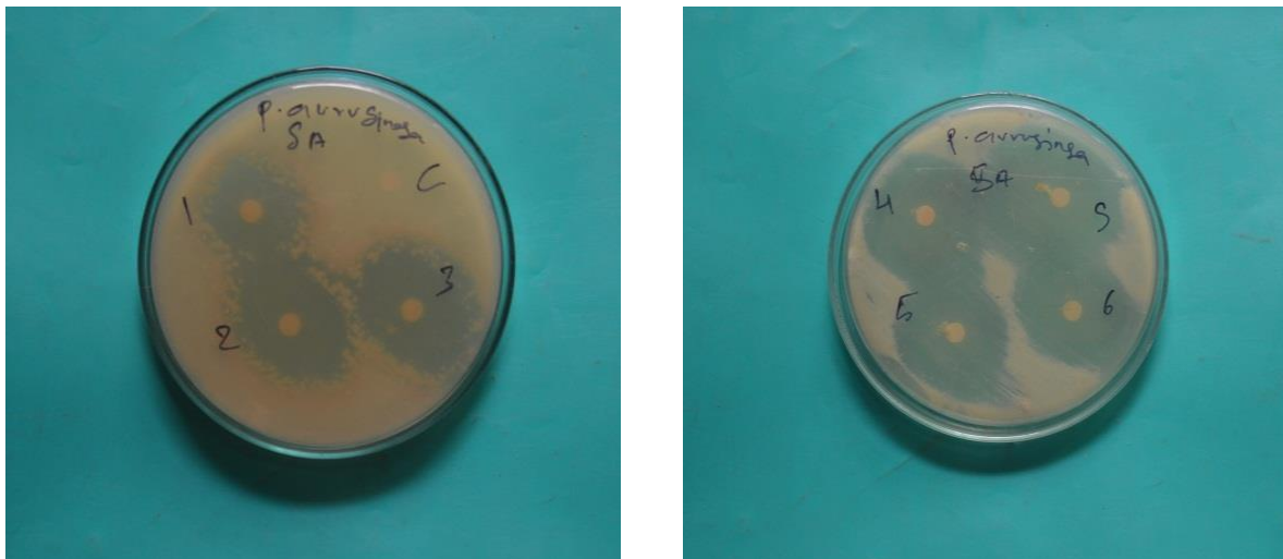
Fig. 1. Petri-plates (1-4) for antibacterial activities of ( E )- N -(4-substitutedbenzylidene)-4-fluorobenzenesulfonamides
