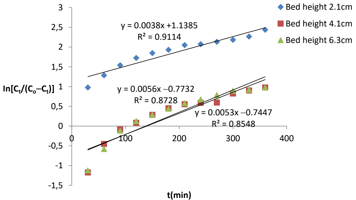
Fig. 9. Yoon-Nelson model plot for the adsorption of metanil yellow on activated palm fibre carbon at various bed heights.
