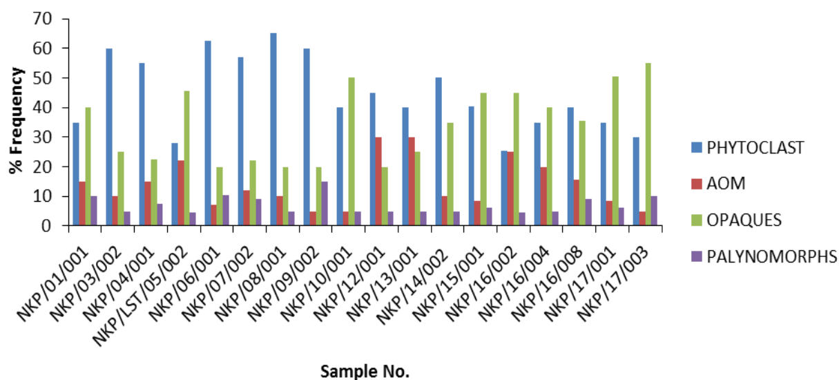
Fig. 4a. Histogram showing the comparism of source rock samples and their percent counts between the Phytoclast, AOM, Opaques and Palynomorphs of the Nkporo Formation samples
