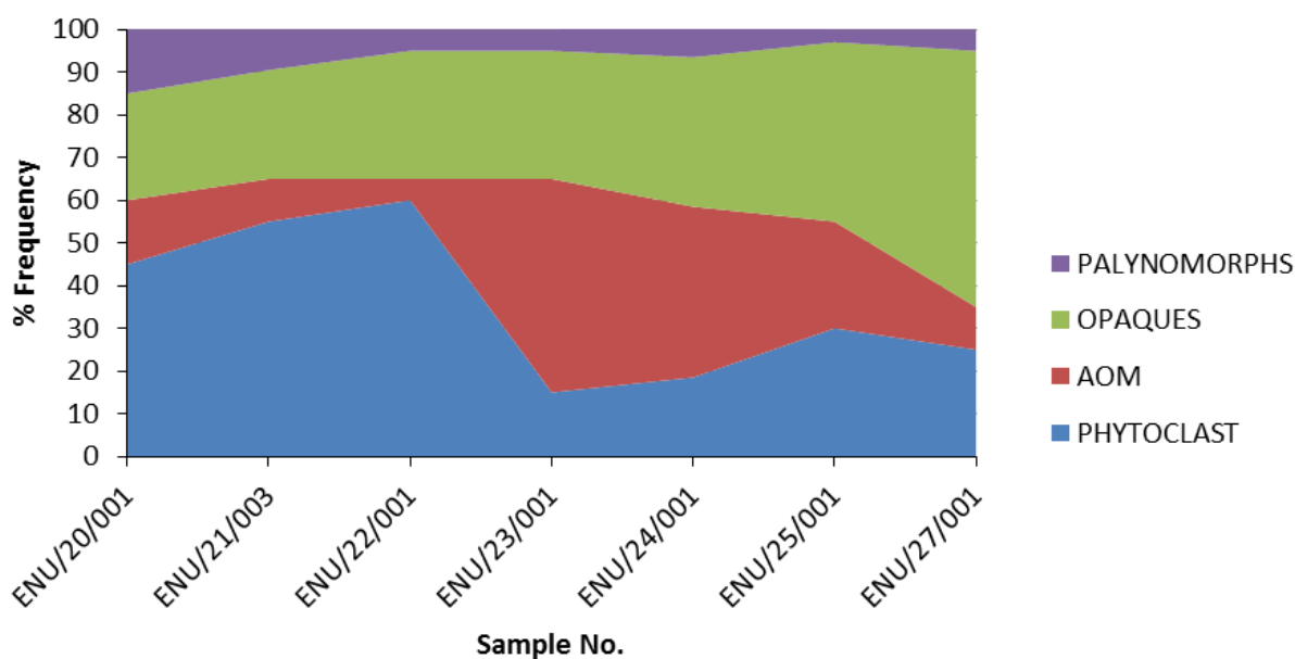
Fig. 5b. Area graph showing their percent counts between the Phytoclast, AOM, Opaques and Palynomorphs of the source rock samples of the Enugu Shale samples
