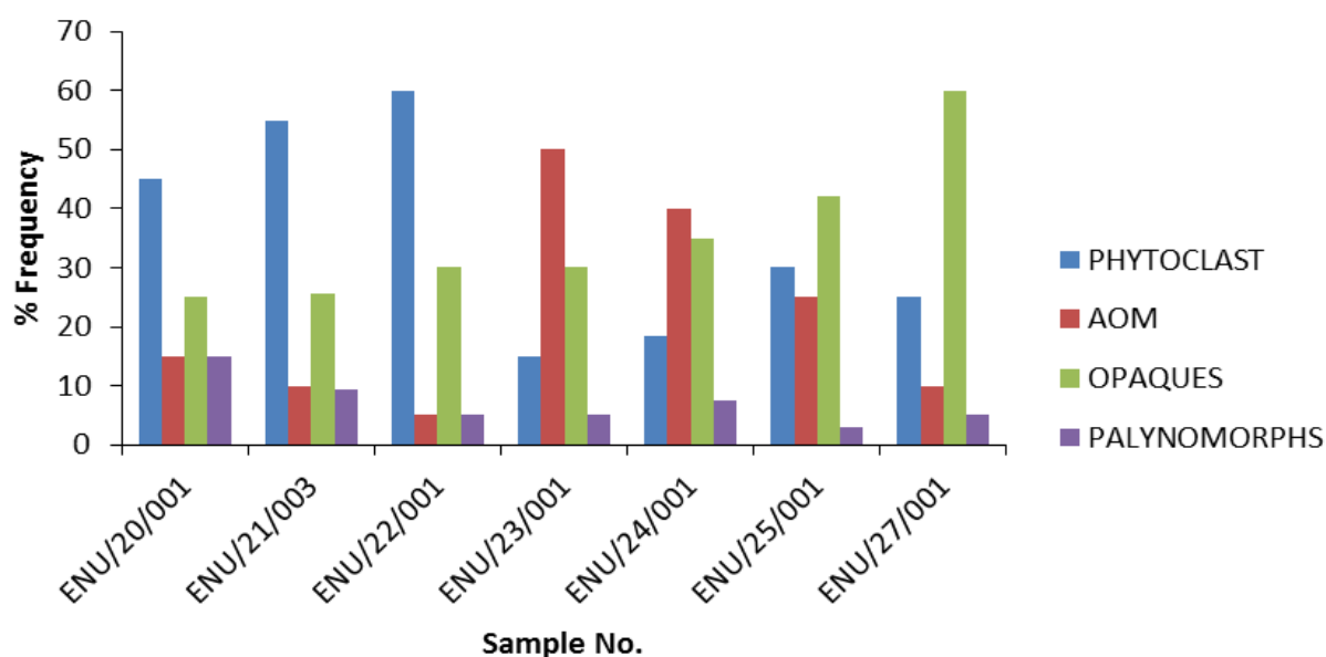
Fig. 4b. Histogram showing the comparism of source rock samples and their percent counts between the Phytoclast, AOM, Opaques and Palynomorphs of the Enugu Shale samples
