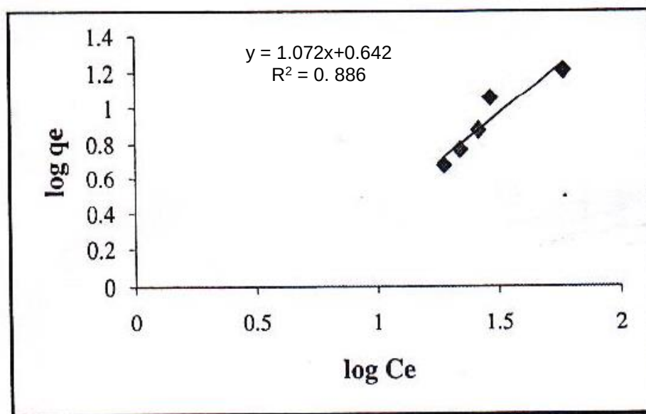
Fig. 6. Freundlich isotherm for the removal of methylene Blue by corn cobs
