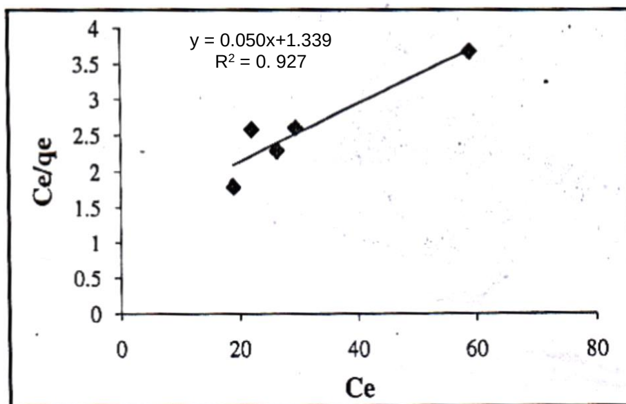
Fig. 5. Langmuir isotherm for the removal of methylene Blue by corn cobs
