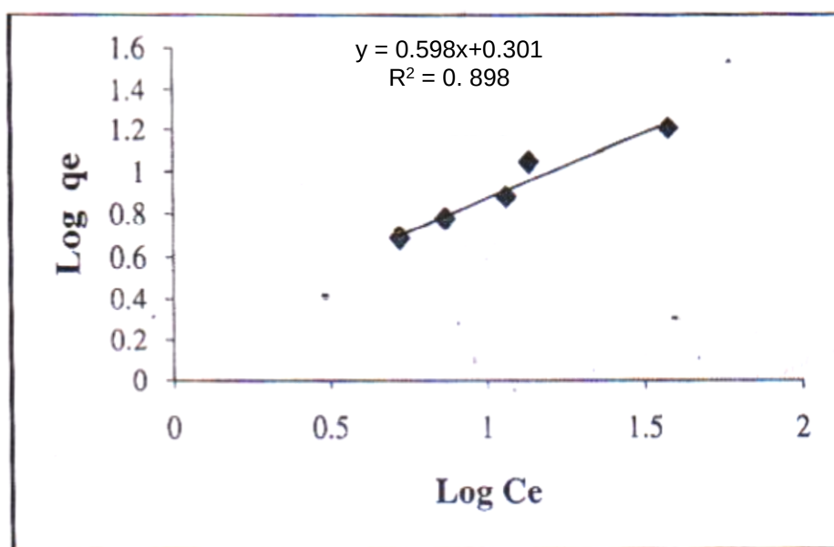
Fig. 4. Freundlich isotherm for the removal of methylene Blue by Animal bone
