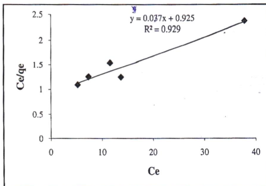
Fig. 3. Langmuir isotherm for the removal of methylene Blue by Animal bone
