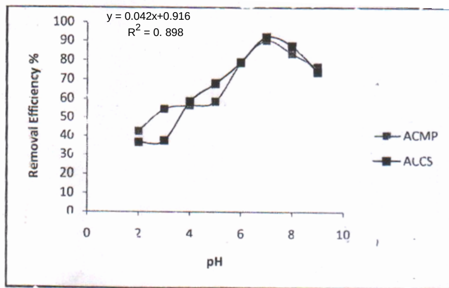
Fig. 2. Effect of pH on Methylene Blue removal
